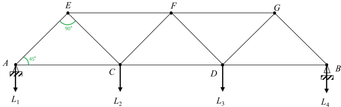
Figure 1: Schematic representation of a bridge (planar truss). Note: assume that both A and B are roller supports.
